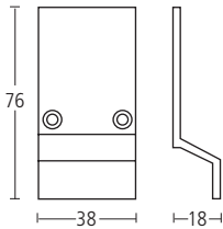
7 76x38x18mm Pull. Finishes: MA • TA
