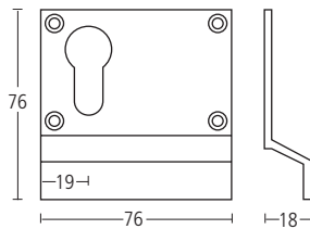
16L/R 76x76x18mm Pull for Euro profile cylinder. STATE HAND. Left hand shown. Finishes: MA • TA
