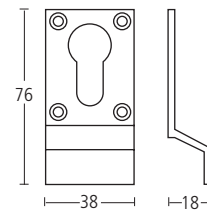
8 76x38x18mm Pull for Euro profile cylinder. Finishes: SS • PS • MA • TA • BS • BD • BL
